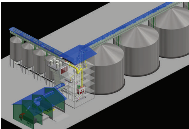
A model of grain Intake, cleaning, drying, bulk loading & storage plant
